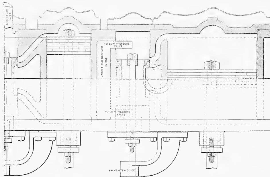
VERTICAL SECTION THROUGH CYLINDERS OF COULTER &amp; MCKENSIE YACHT ENGINE.
